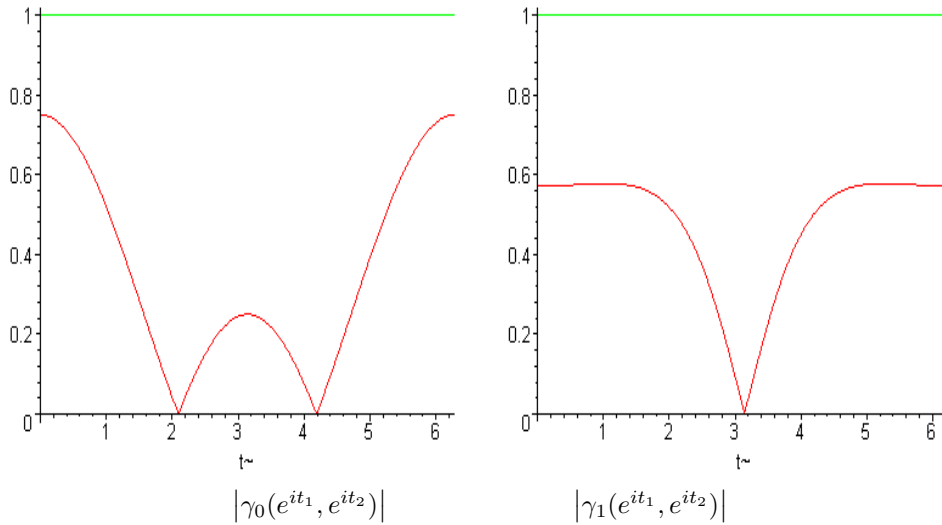
FIG. 1. The absolute values of the functional Schur coefficients for Example 1.
