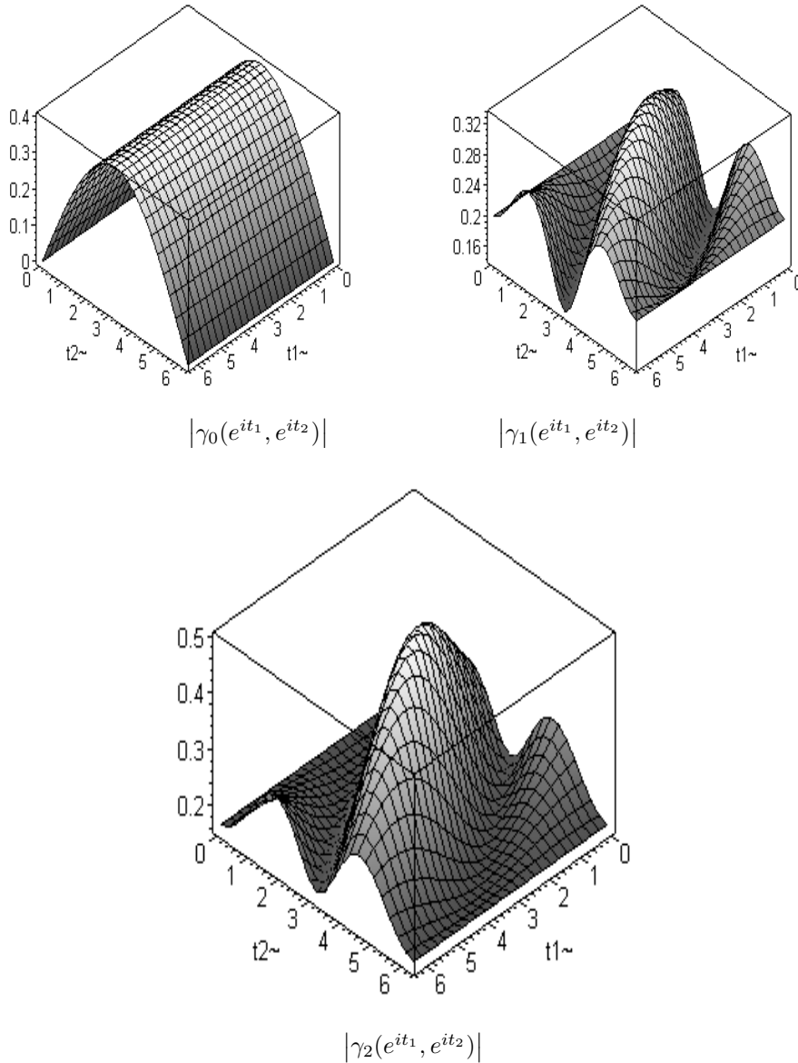
FIG. 4. The absolute values of the functional Schur coefficients for Example 4.
