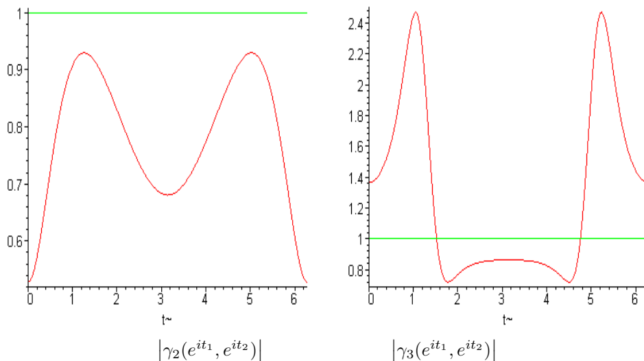
FIG. 2. The absolute values of the functional Schur coefficients for Example 2.
