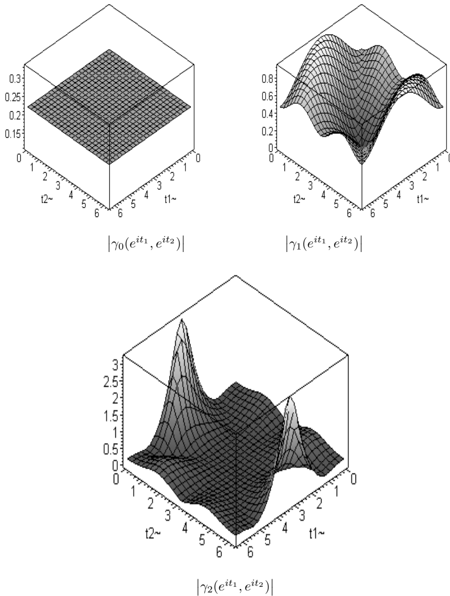
FIG. 3. The absolute values of the functional Schur coefficients for Example 3.
