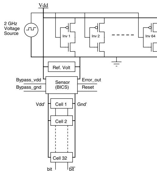
Figure 5. Simulation setup for the noise analysis of the BICS
