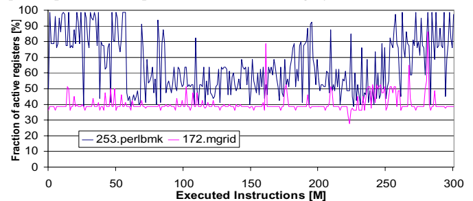
Figure 1. Fraction of active physical registers over the simulation time for the 253.perlbnk and 172.mgrid applications. See Table I for processor configuration.
