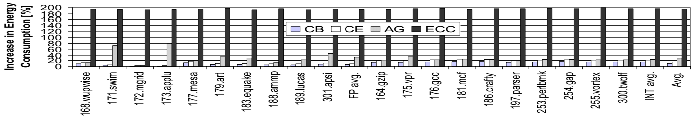
Figure 7. Increase in energy consumption for different schemes. The energy numbers are relative to the consumption in the register file.
