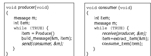
Figure 4. Producer-Consumer Pseudo-Code with 1-element buffer.
