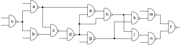
Figure 2: Example circuit.
