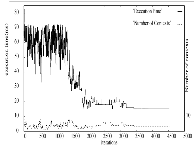
Figure 2. Evolution of execution time and number of contexts in a typical run.
