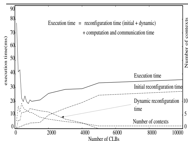
Figure 3. Execution time, reconfiguration times, and number of contexts vs. FPGA size.
