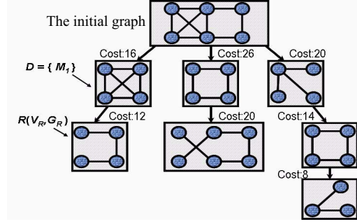
Figure 2. The illustration of the algorithm.
