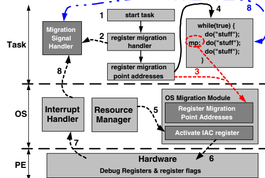
Figure 2. Migrating by using debug registers.
