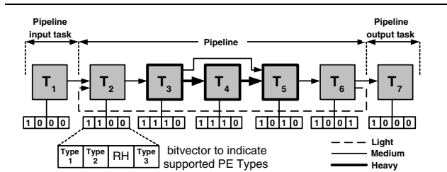
Figure 3. Example application containing a multimedia pipeline (e.g. video decoding).
