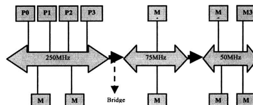
Fig 6: Bus partitioning and frequency assignment for radix benchmark provided by our approach for fitness function a*b.
