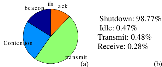
Figure 9: Breakdown of the energy per bit (a) and time (b) spent in the different phases of the protocol
