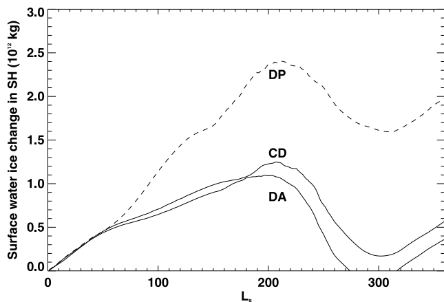
Figure 7. Seasonal variation of total surface water ice south of the equator in a reversed perihelion configuration for the three dust opacity scenarios discussed in section 3.6. The dusty perihelion (DP) scenario yields the largest net deposition of water, with an enhancement factor of 4 and 6, respectively, compared to constant dust (CD) and dusty aphelion (DA) simulations. Variations track each other until approximately Ls 50°, after which date, changes in water transfer from the northern hemisphere become apparent between simulations. The warmer northern tropics of the DP scenario allow additional amounts of water to move south and to condense there. Around Ls 200°, the DA simulation produces the strongest atmospheric warming, and subsequently allows more water return to the northern hemisphere.
