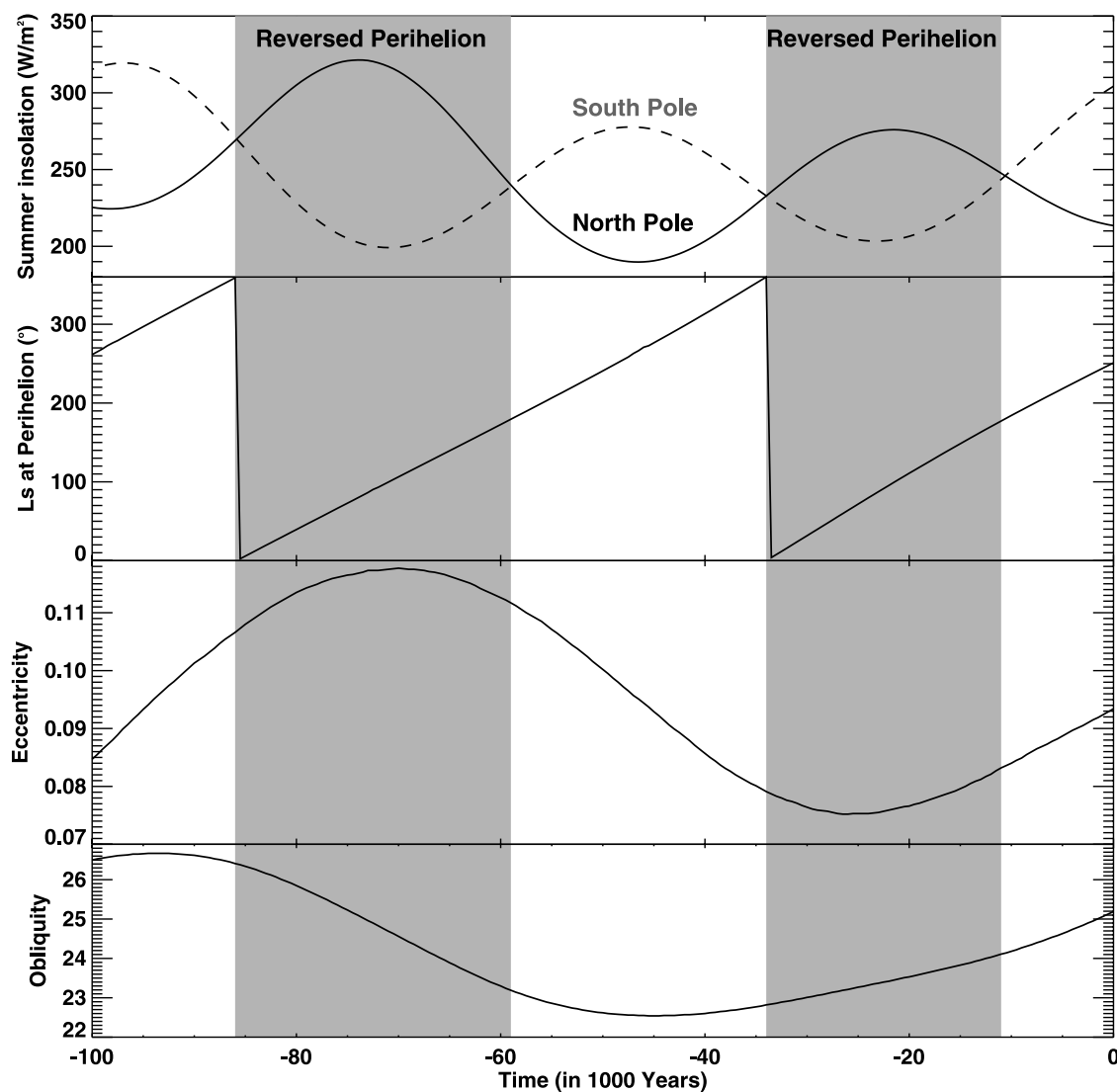
Figure 2. Variations of summer insolation at both poles and corresponding variations of the orbital parameters during the last 100 ka. The reversed perihelion regimes, shown here as the shaded grey portions, bracket periods when the areocentric longitude of perihelion argument ( L_p ) is greater than 0^\circ and smaller than 180^\circ . The shortest modulations of insulations track the secular changes of L_p . A longer-term increase of insolation contrast between the poles is also noted; it is associated with the increase of eccentricity between -20 and -70 ka.
