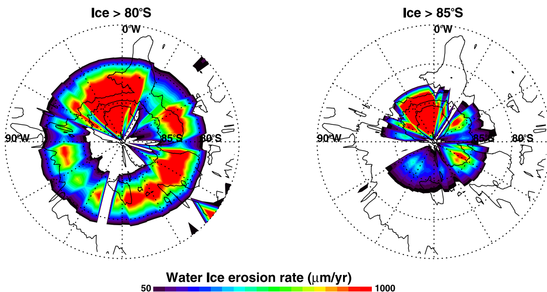
Figure 8. Annual erosion rate of a hypothetical water ice mantle located (left) south of 80°S and (right) south of 85°S predicted by the model under current climatic configuration.
