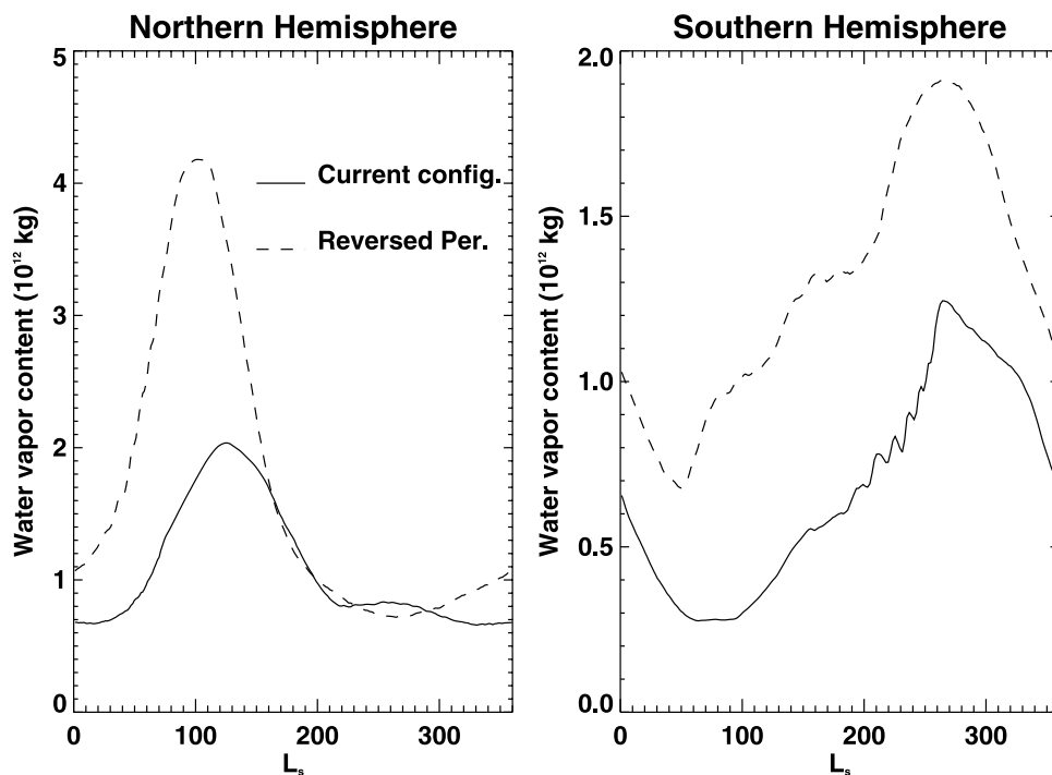
Figure 4. Seasonal variations of integrated water vapor content in each hemisphere for the two opposite perihelion configurations simulated with the model. Increased summer insolation results in a twofold enhancement of the northern water content for the reversed perihelion case. Both simulations fluctuate around a similar level of humidity in fall and start to deviate again after L_s 300^\circ . Southern hemisphere exhibits an annually wetter state compared to present-day simulation.
