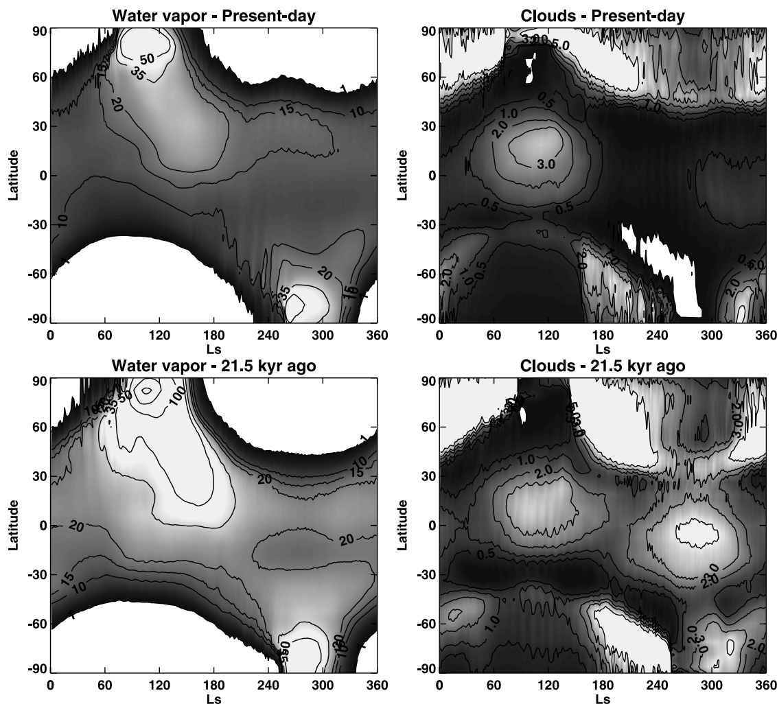
Figure 3. Seasonal and latitudinal distribution of (left) water vapor and (right) water ice clouds for (top) current and (bottom) reversed perihelion configurations. Quantities are expressed in \text{pr } \mu\text{m} .
