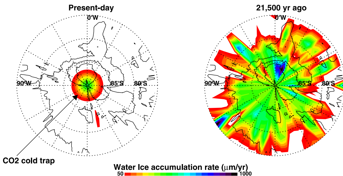
Figure 5. A comparison of water ice accumulation rates predicted by the model in the south polar region for the two perihelion configurations. Present-day map shows net accumulation only at the south pole itself (equivalent to 1 grid point in the model) where the prescription of a CO 2 cold trap forces a local and permanent deposition of water ice. In the reversed perihelion simulation (Figure 5, right), the CO 2 cold trap has been removed and the pattern of accumulation is only controlled by a precipitation versus sublimation positive balance on an annual average.
