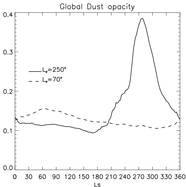
Figure 10. Dust cycle predicted by the Ames GCM for present-day (solid curve, L_p = 250^\circ ) and for a reversed perihelion case (dashed curve, L_p = 70^\circ ). Opacity is given at a wavelength of 9 \mu\text{m} (a multiplicative factor of \sim 2 must be applied to obtain corresponding visible opacity).
