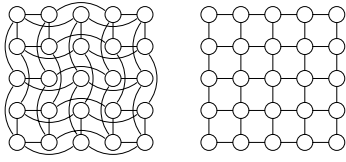
Figure 3: A 5×5 folded torus (left) and a 5×5 mesh (right).
