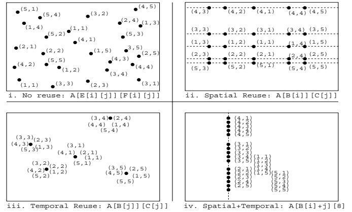
Fig. 2. Examples of compile-time discernible spatial and temporal reuse in indirectly-indexed arrays.
