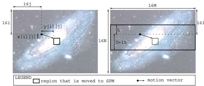
Fig. 1. Migrating the relevant section of an, indirectly-indexed, image-data onto SPM.
