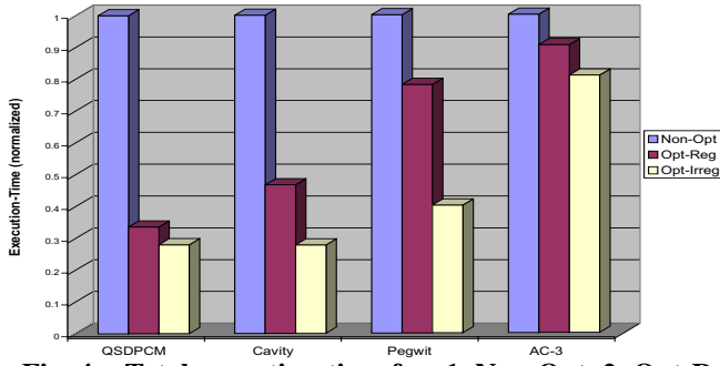
Fig. 4. Total execution-time for- 1. Non-Opt, 2. Opt-Reg, 3. Opt-Irreg.
