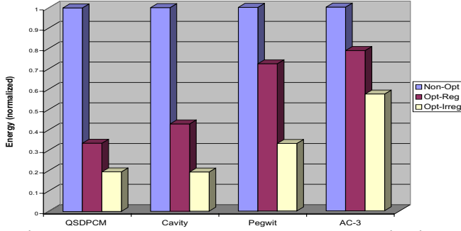
Fig. 5. Total Energy consumed by each application and each version.
