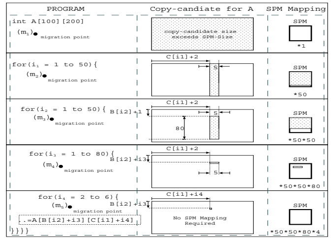
Fig. 3. Trade-off between number of transfers and the size of each transfer.
