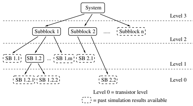
Figure 1. Decomposition of a complex system. Ending nodes in the branches represent subsystems for which no lower-level performance information is needed.
