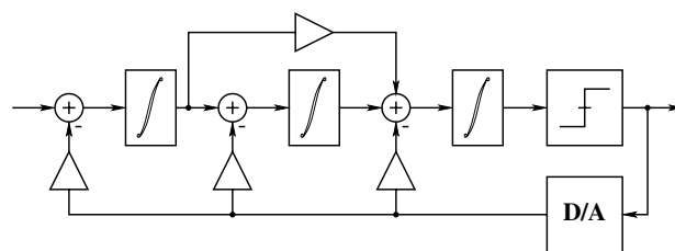
Figure 3. A single-loop 3 th order Delta-Sigma modulator architecture.
