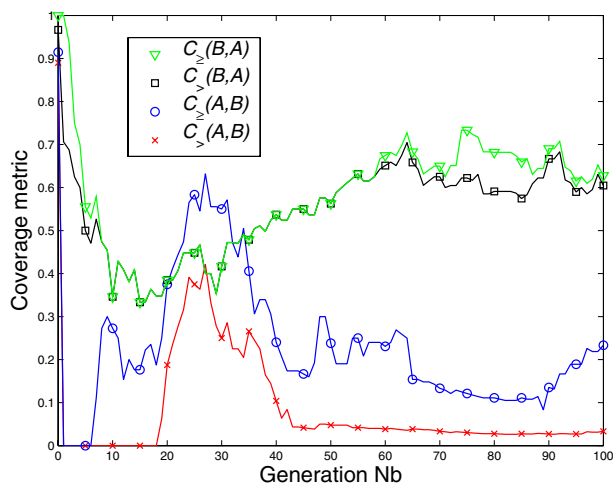
Figure 5. Comparison of \Delta\Sigma Pareto-optimal fronts generated by method A and B, at different generations in the optimization process starting from the initial population, using the coverage metric C .
