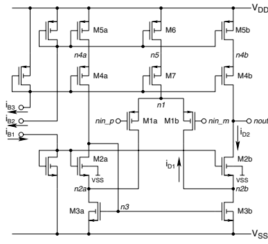
Figure 4. CMOS folded-cascode operational transconductance amplifier.
