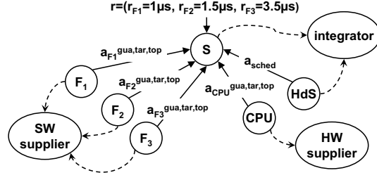
Figure 4. Model of the example system
