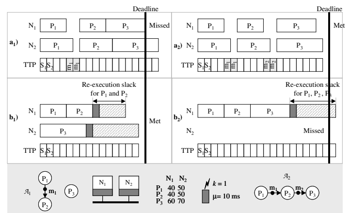
Figure 3. Comparison of Replication and Re-Execution
