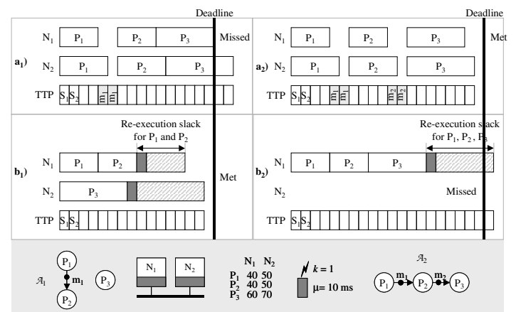
Figure 3. Comparison of Replication and Re-Execution
