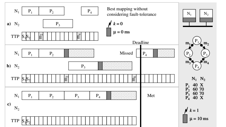
Figure 5. Mapping and Fault-Tolerance
