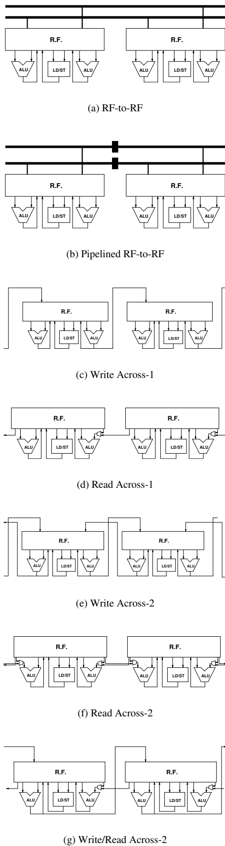
Figure 1. Some Inter-cluster Interconnect Architectures
