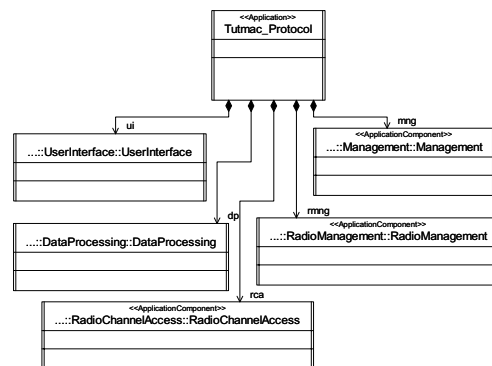
Figure 4. TUTMAC class diagram of an application description.
