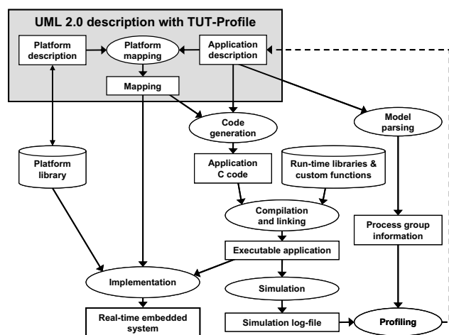
Figure 2. TUT-Profile design and profiling flow.
