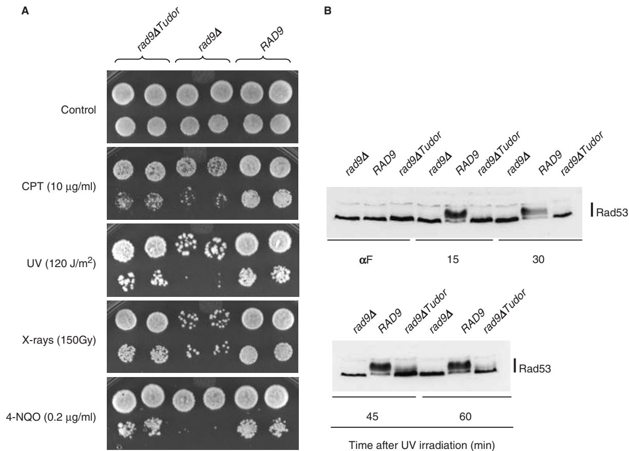
Figure 2. ScRad9[754–947] is required for cell resistance to DNA damage and for Rad53 phosphorylation in G1 phase. (A) rad9Δ ( rad9Δ -L157) transformants containing either an empty vector, the YCp50- Rad9 or the YCp50- Rad9Δ Tudor plasmids were grown to exponential phase in YPD medium and 10-fold serial dilutions were spotted on YPD plates supplemented or not with camptothecin (CPT) or 4-nitroquinoline 1-oxide (4-NQO). Sets of YPD plates were also UV- or X-irradiated. (B) rad9Δ ( rad9Δ -L157) transformants containing either an empty vector, the YCp50- Rad9 or the YCp50- Rad9Δ Tudor plasmids were arrested in G1 with \alpha -factor ( \alpha F), UV irradiated (120 J/m 2 ) and maintained in G1 phase in the continuous presence of \alpha -factor. Aliquots were taken at the indicated times after UV irradiation and analyzed by western blotting using anti-Rad53 antibodies.
