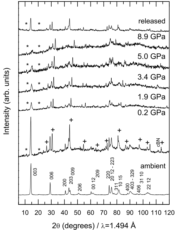
FIG. 5: Neutron powder diffraction patterns of \text{CsC}_8 as a function of pressure with NaCl (+) as pressure transmitting medium and pressure marker. The two stars (*) indicate additional peaks (see text). The ambient diffraction pattern was taken in a vanadium container. The released pressure diffraction pattern was recorded in the press after the HP cycle.
