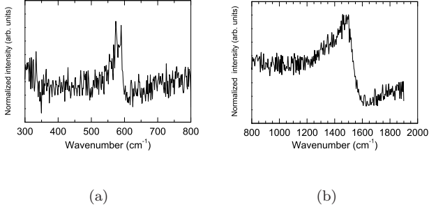
FIG. 7: High- (b) and low- (a) frequencies Raman signal of \text{CsC}_8 at ambient pressure and room temperature with a 632.8 nm laser excitation.
