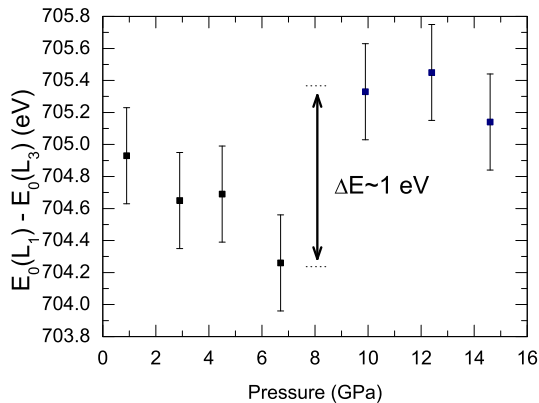
FIG. 13: Difference between the energy of the L_1 - and L_3 -Cs edges in \text{CsC}_8 as a function of pressure.
