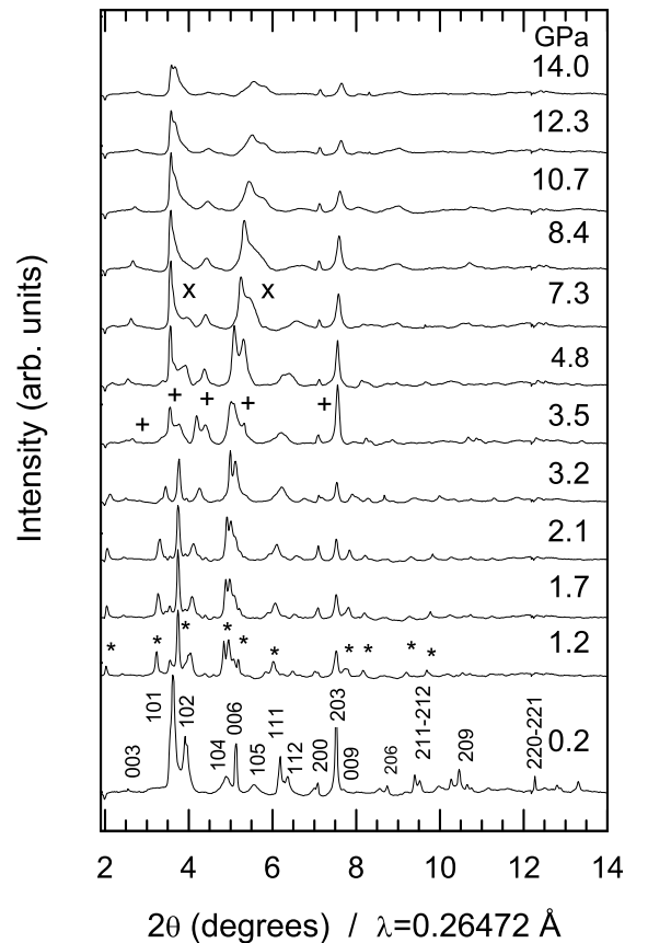
FIG. 2: Selected X-ray diffraction patterns of the CsC 8 compound as a function of pressure. Pressure in GPa is given at the right side of each curve. The first pressure pattern corresponds to the hexagonal structure (CsC 8 -I). The sample was confined in oil as pressure transmitting medium. Intensity was normalized for all patterns to the same counting time. Stars (★), plus (+) and crosses (×) symbols show the appearance of new Bragg peaks corresponding to CsC 8 -II, CsC 8 -III and CsC 8 -IV phases respectively (see Table III).
