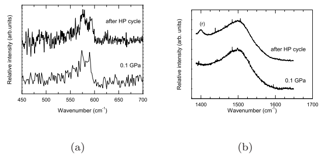
FIG. 11: Comparison of the low- (a) and high-frequencies (b) Raman spectrum of \text{CsC}_8 between the first pressure point at 0.1 GPa in the DAC and after the HP cycle to 8.2 GPa. Fluorescence of ruby is indicated by the (r) label.
