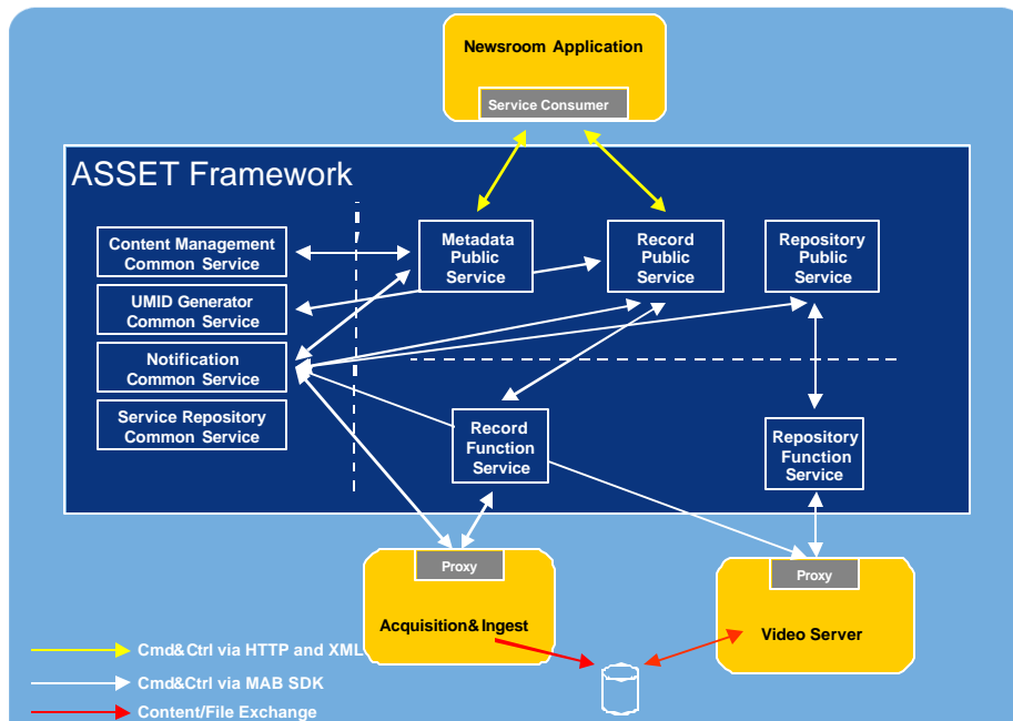
Figure 3 – ASSET demonstration platform components
