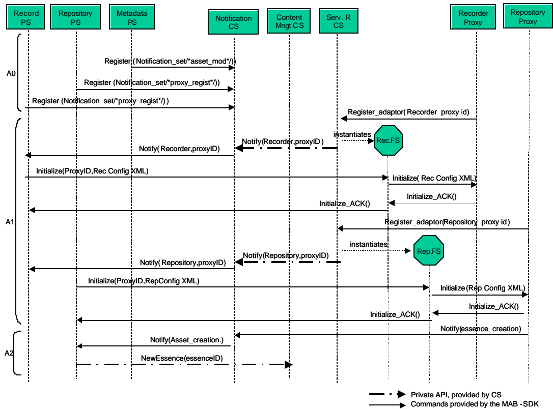
Figure 5 – ASSET demonstration Registration Scenario
