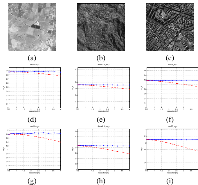
Fig. 3. (a)-(c) Three images ( \copyright CNES); (d)-(f) graphs of m_1(q, r, t)/r (with q = 0 ) as a function of r ; (g)-(i) graphs of m_2(q, r, t)/r^2 (with q = 0 ) as a function of r . On all these graphs, solid lines correspond to the case where r^2\sqrt{t^2 + p^2} is kept constant (with p = 1.3 ), and dashed lines correspond to the case where rt is kept constant.
