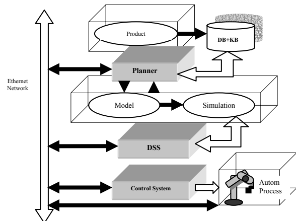
Fig. 2. Integrating DSS in the process control
