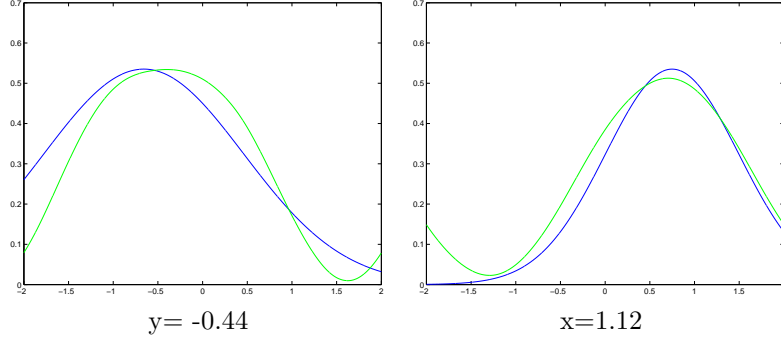
FIGURE 2. Sections for the process AR(i) observed through a Laplace noise, n = 500
