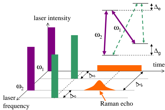
FIG. 3: (color online) Raman echo pulse sequence for photon echo elimination using the two \Lambda -systems. The second pulse is detuned from the first one by the excited state splitting \Delta_e but still satisfies the two-photon resonance. Inset: 4-level system. The first and second pulse frequencies (\omega_1, \omega_2) and (\omega_1 + \Delta_e, \omega_2 + \Delta_e) are respectively depicted in solid and dashed arrows.
