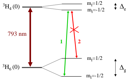
FIG. 1: (color online) Nuclear Zeeman effect in Tm:YAG. Nuclear spin selection rule forbids transition 2.
