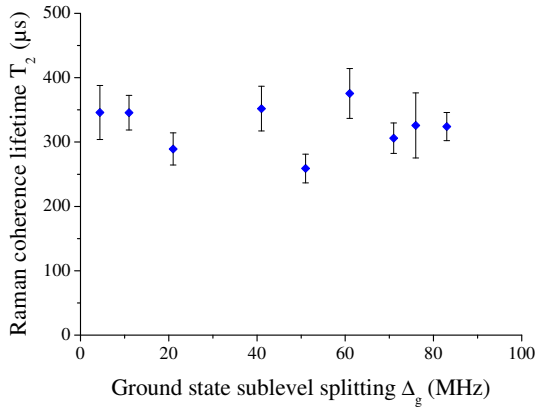
FIG. 5: Measurement of the spin coherence lifetime for different ground state splittings, from 4 to 83 MHz. The error bars correspond to the standard error deduced from a least-squares fit.
