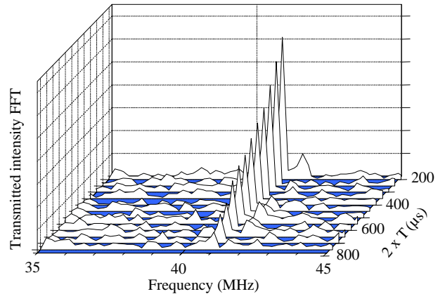
FIG. 4: (color online) Raman echo signals for \Delta_g = 41 MHz as delay time T is increased from 100 \mu\text{s} to 400 \mu\text{s} . The spin coherence lifetime is derived from the exponential decay of this signal.
