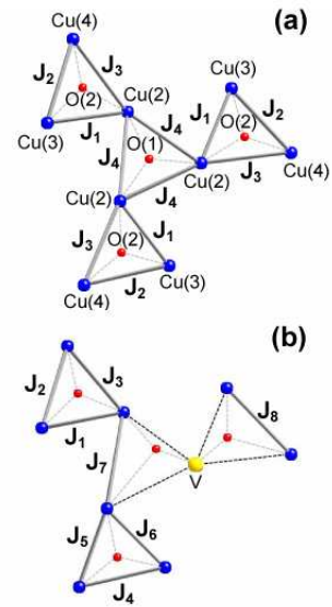
FIG. 3: DFT calculated positions of the Cu (blue circles), V (large yellow circles), and O (small red circles) atoms in the 9-spin clusters (a) and 8-spin clusters (b). The labeling of the different superexchange interactions is used in section III A.
