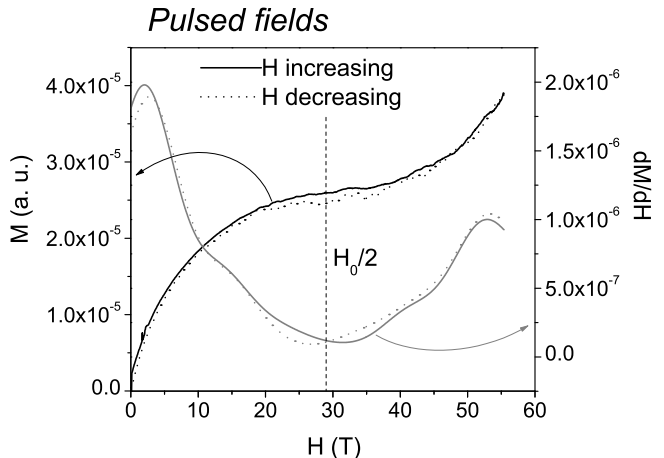
FIG. 6: Magnetization isotherm measured around T=1.4 K in increasing and decreasing pulsed field up to 55 T, and its field derivative. The dotted line indicates the middle of the magnetization plateau, which is related to the Zeeman crossing of the two first levels of the system with \Delta S=+1 (see inset of Fig. 7).
