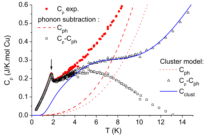
FIG. 8: Specific heat measurements at low temperature (circles) analyzed with two models: (i) The phonon contribution (dashed line) is obtained from a fit of C_p/T as a function of T^2 using the low temperature approximation C_p = \beta_1 T^3 + \beta_2 T^5 in the range [12-28 K]. The resulting magnetic signal is represented with square symbols. (ii) The second model is based on the multi- J spin cluster description reported in table III of section III. The lattice contribution of the form C_p = \beta_1 T^3 + \beta_2 T^5 (dotted lines) is adjusted such that the remaining signal (triangles) coincides with the calculated magnetic specific heat (solid line) above 5 K.
