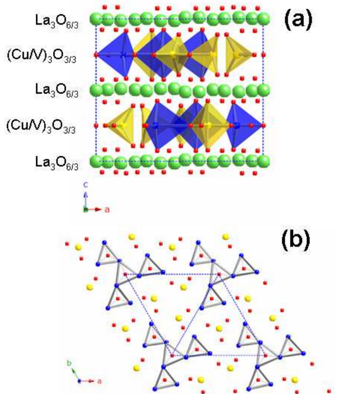
FIG. 1: (a) \text{La}_3\text{Cu}_2\text{VO}_9 structure projected along the b axis: \text{LaO}_{6/3} layers alternating with (\text{Cu/V})\text{O}_{3/3} ones with the O polyhedron drawn around Cu and V atoms. (b) \text{La}_3\text{Cu}_2\text{VO}_9 structure projected along the c axis: (\text{Cu/V})\text{O}_{3/3} layers showing the 9 \text{Cu}^{2+} clusters at the vertices of a triangular lattice. La, V, Cu and O atoms are represented by large green, yellow, blue and small red circles, respectively.
