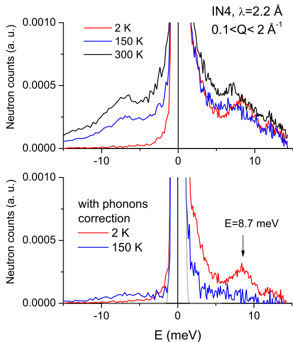
FIG. 9: Inelastic neutron scattering measurements. Upper frame: Energy spectra at 2, 150 and 300 K, integrated on the Q interval [0.1, 2] \text{ \AA}^{-1} . Lower frame: 2 and 150 K spectra corrected from the phonon contribution using the 300 K spectrum (see text).
