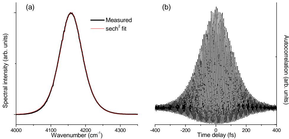
Figure 2: (a) Spectrum (FWHM: 76\text{ cm}^{-1} ) and (b) interferometric autocorrelation (FWHM: 250 fs) of a 130-fs pulse of the \text{Cr}^{2+}:\text{ZnSe} mode-locked laser. Pump power: 1.9 W, output power: 50 mW, repetition rate 200 MHz.
