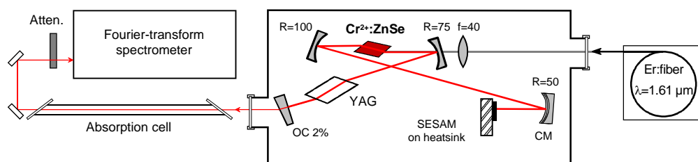
Figure 1: Experimental set-up. CM: chirped mirror. OC: output coupler. Atten: attenuator.
