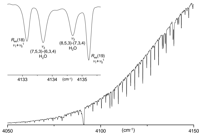
Figure 3: Part of a \text{C}_2\text{H}_2 spectrum at 0.12\text{ cm}^{-1} resolution in the 2.4\text{ }\mu\text{m} region. The baseline modulation is not noise-related but due to a channel spectrum from an unwedged window. The strongest spectral features are the P , Q and R branches of the \nu_1 + \nu_5^1 band [12] of ^{12}\text{C}_2\text{H}_2 , centered at 4090\text{ cm}^{-1} . The intensity alternation is obvious in the R -branch. The upper left inset is a zoom showing acetylene and residual water vapor lines coming from a 5 meters air path between the cell and the interferometer. The \text{H}_2\text{O} lineshapes reveal an atmospheric-pressure broadening. The rotational assignment for the \text{H}_2\text{O} lines [13] gives (J, K_a, K_c) .
