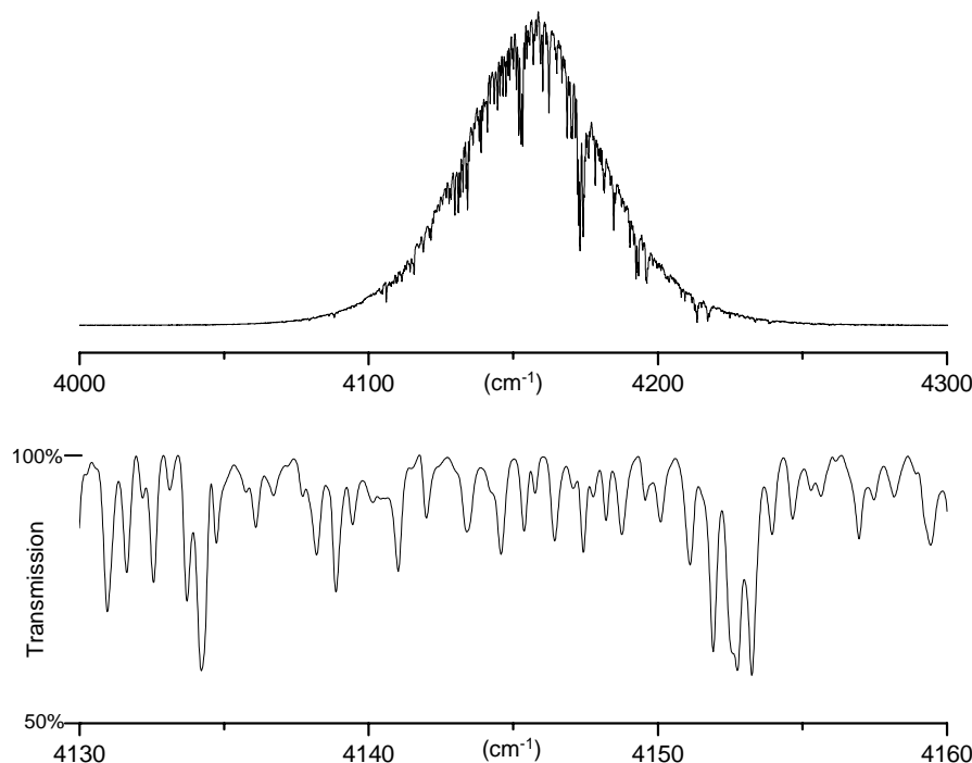
Figure 4: Spectrum of \text{NH}_3 in the 2.4 \mu\text{m} region illustrating the spectral bandwidth and SNR capabilities of the spectrometric technique. The \nu_1 + \nu_2 and \nu_2 + \nu_3 combination bands are observed. The upper part of the figure shows the whole spectral domain covered in a single recording while the lower part shows a portion expanded in wavenumber and intensity scales.
