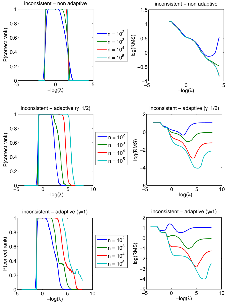
Figure 4: Synthetic example where consistency condition in Eq. (7) is not satisfied: probability of correct rank selection (left) and logarithm of the expected mean squared estimation error (right), for several number of samples as a function of the regularization parameter, for regular regularization (top), adaptive regularization with \gamma = 1/2 (center) and \gamma = 1 (bottom).
