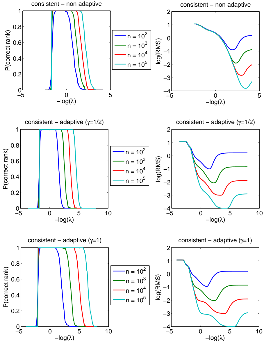
Figure 3: Synthetic example where consistency condition in Eq. (8) is satisfied: probability of correct rank selection (left) and logarithm of the expected mean squared estimation error (right), for several number of samples as a function of the regularization parameter, for regular regularization (top), adaptive regularization with \gamma = 1/2 (center) and \gamma = 1 (bottom).
