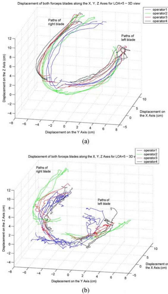
Fig. 8. Paths of the forceps blade tips for experts (a) and for novices (b).
