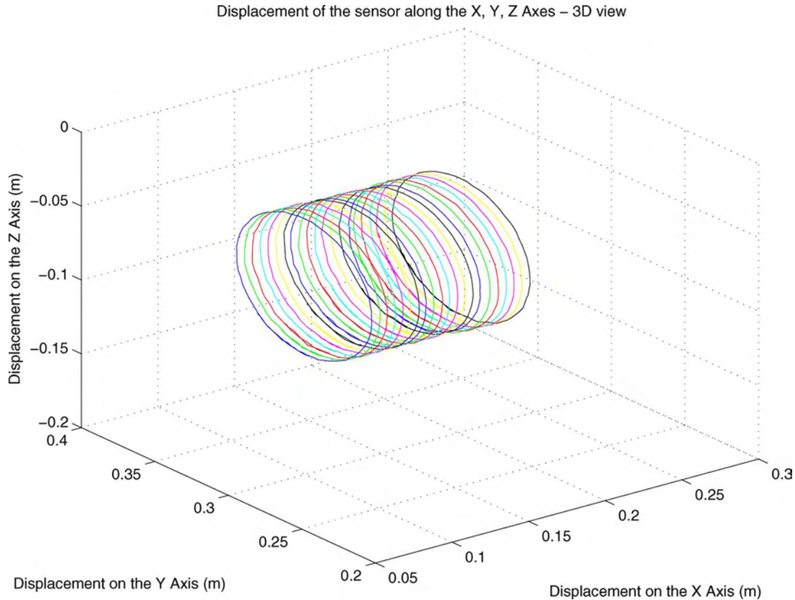
Fig. 3. Measurements of the sensor displacement on separated circles of 0.5 cm along the \vec{x} -axis.
