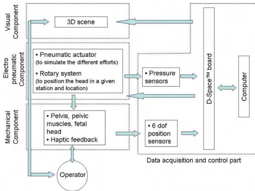
Fig. 1. Principle diagram of the BirthSIM simulator.
