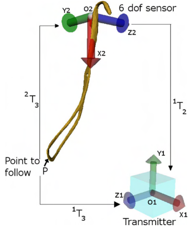
Fig. 6. Different frames associated with the forceps.
