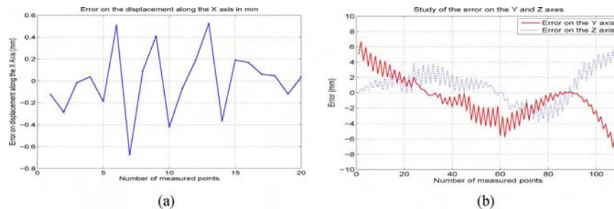
Fig. 4. Sensor errors along the three axes. (a) Sensor static errors along the \vec{x} -axis. (b) Sensor dynamic errors along the \vec{y} - and \vec{z} -axes.
