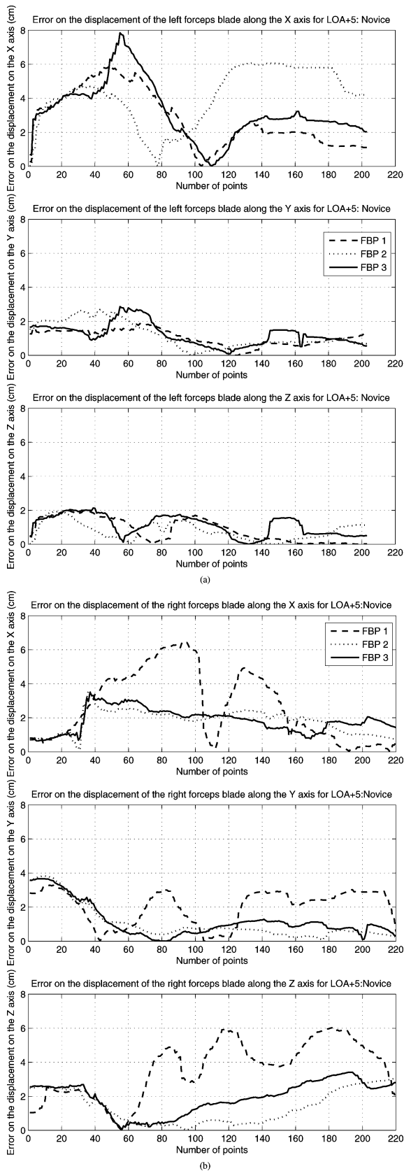
Fig. 10. Errors of a novice during the FBP along the \vec{x} , \vec{y} and \vec{z} axes. (a) Left blade error during its placement. (b) Right blade error during its placement.
