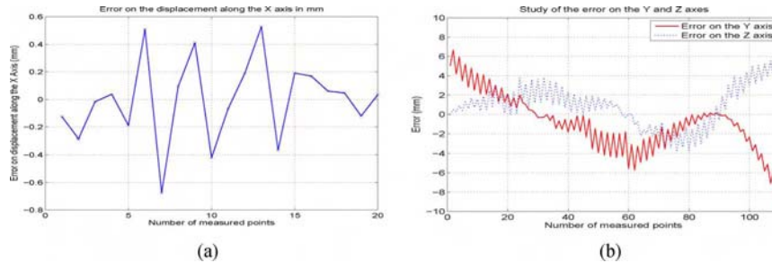
Fig. 4. Sensor errors along the three axes. (a) Sensor static errors along the \vec{x} -axis. (b) Sensor dynamic errors along the \vec{y} - and \vec{z} -axes.
