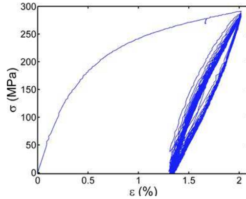
Fig. 9 Cu–Al–Be(2) quasistatic cyclic test at 22^\circ\text{C}
