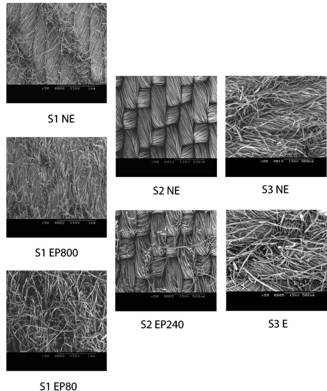
Fig. 2 Photographs of the tested twill fabrics.
