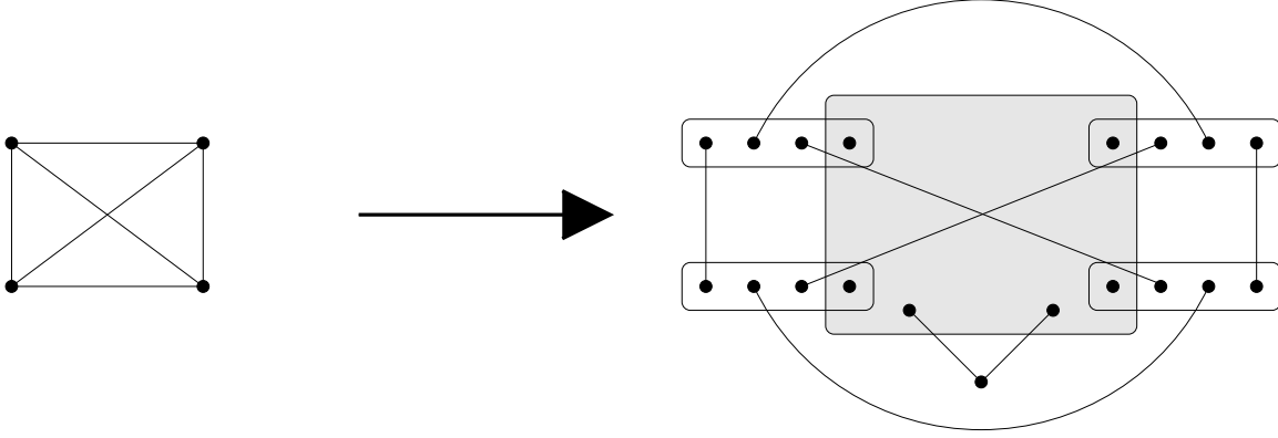
Figure 6: An example of the construction from a K_4 .
