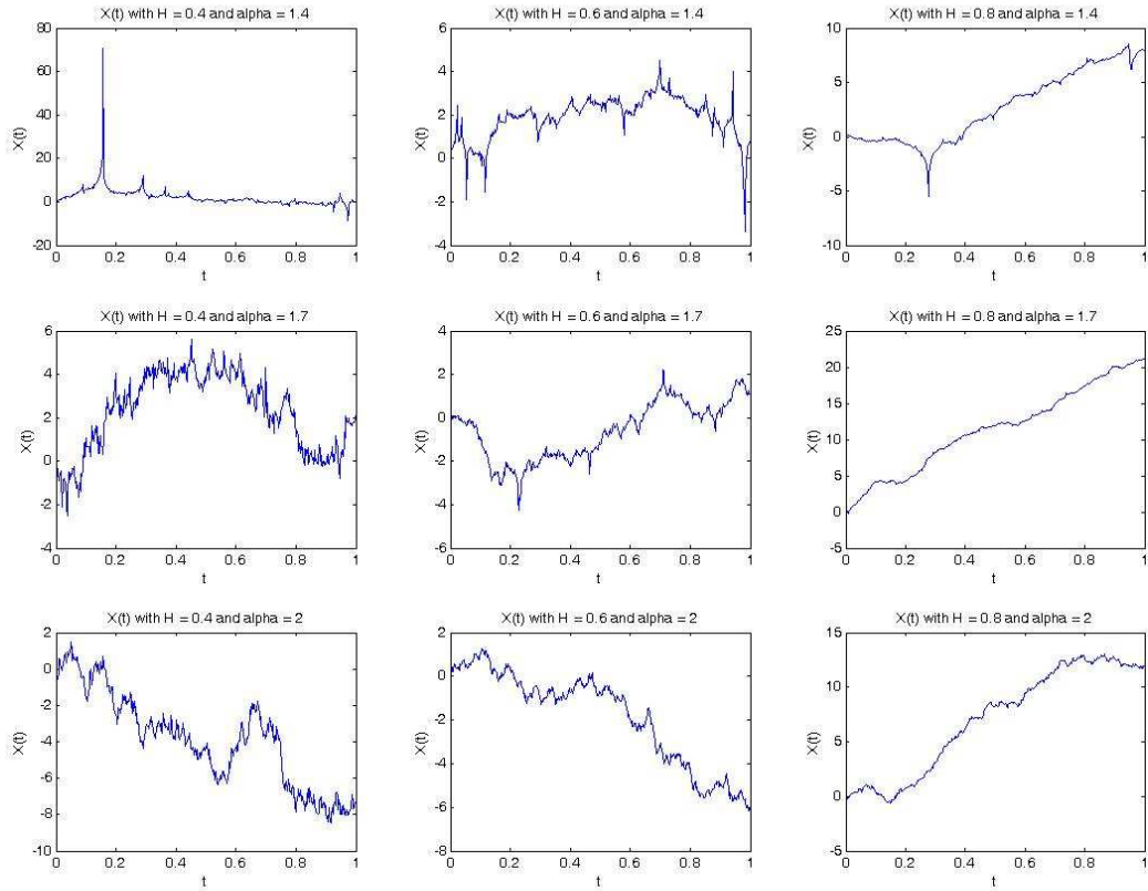
FIGURE 1. Approximations of LFSM sample path for various H, \alpha . We used A = 101 and L = 2^{18} and N = M = 2^{16} .
