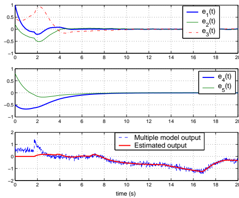
Fig. 1. Estimation error (top and center), measured and estimated output (bottom)
