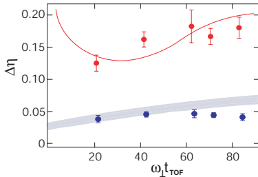
FIG. 3: Time evolution of the measured density modulations \Delta\eta during a TOF for \gamma = 0 (no disorder; blue points) and \gamma = 0.41 (with disorder, red points). The shaded area corresponds to the calculation of [17] taking into account the uncertainty on the temperature. The solid red line is the result of numerical calculations for \gamma = 0.4 (see text).
