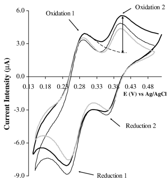
Fig. 1. Voltammograms ( \text{Si}(\text{OH})_4=145 \mu\text{M} , molybdate= 10 \text{ mM} and \text{pH}=1.5 ) at a gold electrode (bold black line), a platinum electrode (thin black line) and a glassy carbon electrode; scan rate= 200 \text{ mV/s} . Extrapolation is represented by the dotted curve, according to Cottrell's law.
