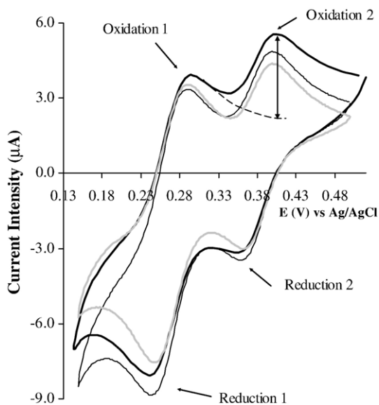
Fig. 1. Voltammograms ( \text{Si}(\text{OH})_4=145 \mu\text{M} , molybdate=10 mM and pH=1.5) at a gold electrode (bold black line), a platinum electrode (thin black line) and a glassy carbon electrode; scan rate=200 mV/s. Extrapolation is represented by the dotted curve, according to Cottrell's law.
