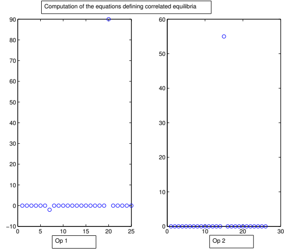
FIG. 6 – Aumann's conditions unsatisfied for external regret minimization.
