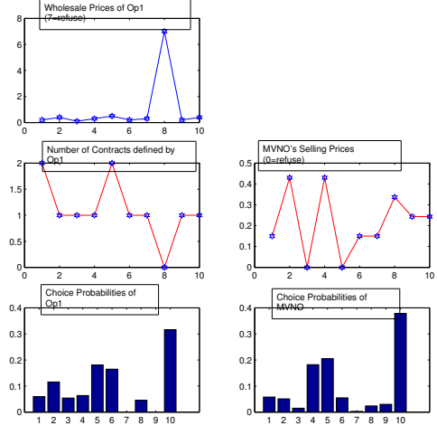
FIG. 12 – Probabilities of MVNO agreement's selection for Op1 and Op2.
