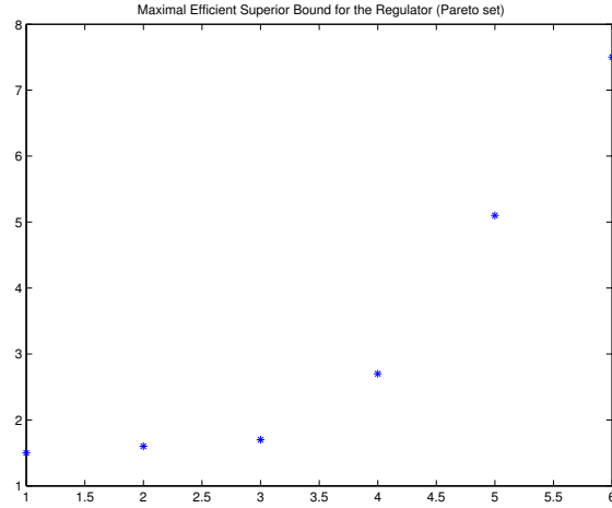
FIG. 13 – Efficient upper bounds for the MVNO agreement, fixed by a regulatory authority.
