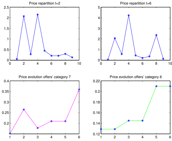
FIG. 7 – Dynamic evolution of the mean market prices.
