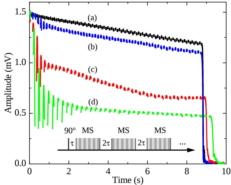
FIG. 3: [color online] Spin echo trains: Traces (a) - (d) correspond to echo trains that are observed when RMS sequences with delay times \tau = 16, 24, 32 , and 40 ms, respectively, are applied to the magnetized liquid. The MS cycles used to obtain these data are identical to those described in the caption of Fig. 2 except for the facts that each one terminates with an additional 180_y^\circ rotation (cf. trace (c) of Fig. 2) to refocus interactions linear in \mathbf{M} , and that the symmetry of alternate MS cycles is inverted to reduce the accumulation of phase errors. That is, odd MS cycles are of the form [90_y^\circ, n \times (360_x^\circ, -360_x^\circ), 90_y^\circ] while even MS cycles are of the form [-90_y^\circ, n \times (-360_x^\circ, 360_x^\circ), -90_y^\circ] . These data were acquired at T \sim 1.1 K, with X \sim 4.5 % and B_{\text{dip}} \sim 0.8 \mu\text{T} . In the limit B_{\text{dip}} \rightarrow 0 , CPMG-based measurements yield D \sim 2 \times 10^{-7} \text{m}^2/\text{s} .
