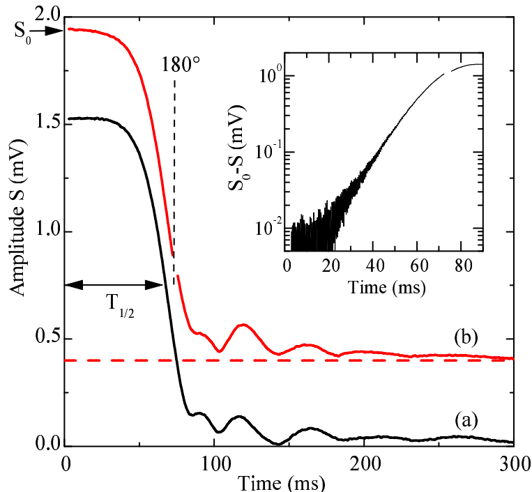
FIG. 1: [color online] FID response of polarized ^3\text{He} in liquid ^4\text{He} (a) to a 90^\circ rf tipping pulse and (b) to a 90^\circ - \tau - 180^\circ sequence. The time at which the FID amplitude S drops to half of its initial value S_0 is denoted T_{1/2} , which is of order 70 ms for these examples. Trace (b) has been displaced upward by 0.4 mV for the sake of clarity. The inset shows the deviation of trace (b) from its initial amplitude. These data were acquired at T = 1.14 K, with X \sim 2\% and B_{\text{dip}} \sim 0.9 \mu\text{T} for trace (a) and X \sim 5\% and B_{\text{dip}} = 0.7 \mu\text{T} for trace (b).
