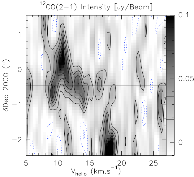
Fig. 5. ^{12}\text{CO } J=2-1 position–velocity diagram in the North–South direction through RW Aur B, illustrating the asymmetry in velocity and spatial extension of the associated molecular peak. The horizontal line shows the declination of RW Aur B. The vertical line indicates the RW Aur A average systemic velocity. The bright region at ( 19 \text{ km s}^{-1} , -2.4'' ) is the redshifted arm. The data cube was smoothed by a 1'' Gaussian in RA to increase the S/N ratio. Contour spacing is 18 \text{ mJy/beam} ( 1.5\sigma in the smoothed cube).
