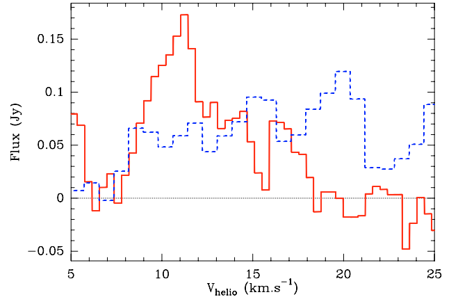
Fig. 6. ^{12}\text{CO} spectra towards RW Aur B. Continuum emission is subtracted. The solid histogram displays the J=2-1 spectrum, integrated over the J=1-0 beam ( 2.42'' \times 1.55'' at \text{PA} = 24^\circ ). The dashed histogram displays the J=1-0 spectrum, multiplied by 4 (the 3\sigma level is then 0.12 \text{ Jy} ). The emission component at 11 \text{ km s}^{-1} appears partly optically thin.
