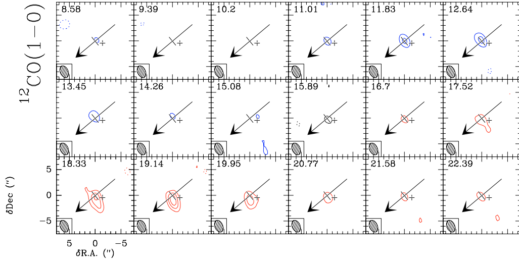
Fig. A.1. Channel maps of ^{12}\text{CO } J = 1-0 towards RW Aur, rebinned to a spectral resolution of 0.85 \text{ km s}^{-1} . Radial velocities ( heliocentric ) are given in the upper left corner of each panel. The large cross indicates the position of RW Aur A, with an arrow pointing in the blue jet direction. The small cross indicates the position of RW Aur B. Blue and red contours respectively indicate blue and red-shifted channels with respect to the RW Aur A mean heliocentric velocity ( V_{\text{helio}} \approx 15.87 \pm 0.55 \text{ km s}^{-1} , Gahm et al. (1999)). Contour levels correspond to -3, 3, 6 and 9 \sigma with 1\sigma = 10 \text{ mJy/Beam} = 0.24 \text{ K} (see Table 1 for details). Dotted lines show negative contours. The hatched ellipse represents the beam FWHM size, 2.42'' \times 1.55'' at \text{PA} = 24^\circ . Continuum is not subtracted.
