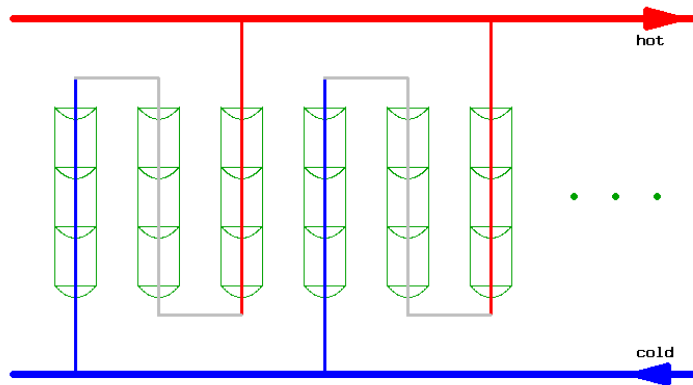
Figure 6: Primary circuits
