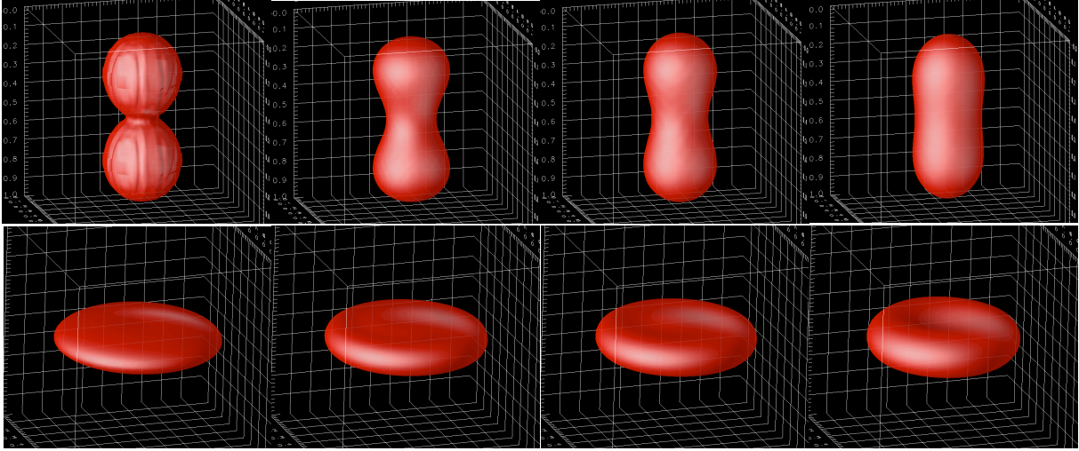
FIGURE 1: Shape optimization for equilibrium shapes of biological shapes. Top pictures: \eta = 0.8 , bottom pictures: \eta = 0.586 . Initialization to steady-state from left to right. Computations made by Thomas Milcent.
