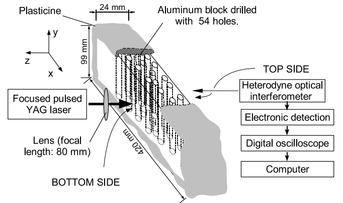
FIG. 2: Experimental setup : The propagation medium is an aluminum block drilled with 54 vertical cylindrical holes (diameter: 4 mm). A Q-switched Nd:YAG laser shoots on the bottom side 100 pulses (24 ns duration and 280 MW/cm 2 intensity each). On the top side a heterodyne interferometer senses the vertical displacement of the aluminum/air interface. This measure is repeated at 7 different locations ( X_0 = 0 mm \rightarrow X_6 = 60 mm) for each source position. Plasticine was stuck on the edges and the four lateral sides to mimic absorbing boundary conditions and avoid the generation of Rayleigh waves by mode conversion at the edges.
