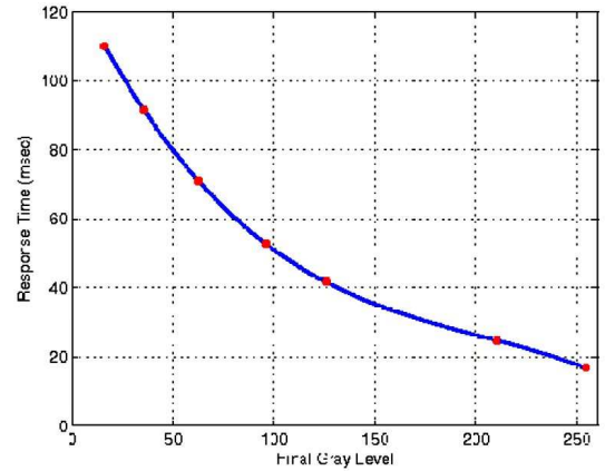
Figure 4: Estimation of response time for rising transitions in \uparrow T_0 with polynomial approach (blue) initialized by 7 measurements (red).
