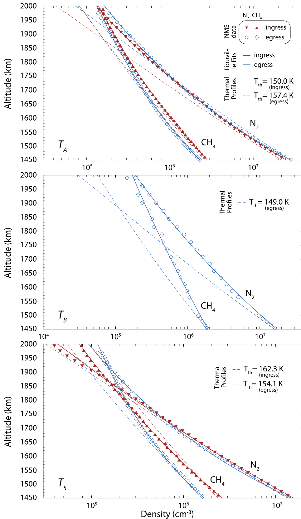
Figure 7. Results of the fit of the \text{N}_2 and \text{CH}_4 density data recorded by INMS in Titan’s exosphere during flybys T_A , T_B , and T_5 , using the method presented by Schunk and Nagy [2000] based on the Liouville theorem. The thermal profiles are represented with dash lines and the fit profiles with solid lines (red for ingress and blue for egress).
