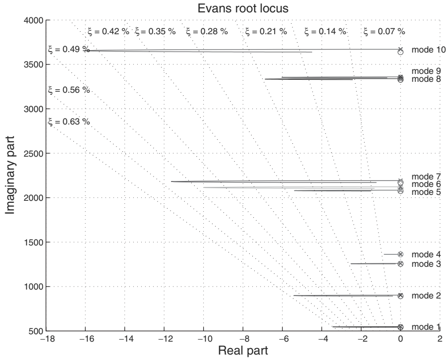
Figure 9. Evans root locus: mechanical modes (—) and zeros.
