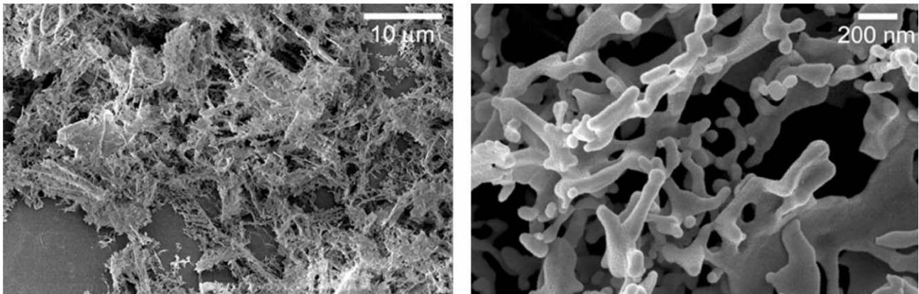
Fig. 1 Morphology at different scales of the \text{La}_{9.33}\text{Si}_6\text{O}_{26} nanopowders as obtained after calcination.
