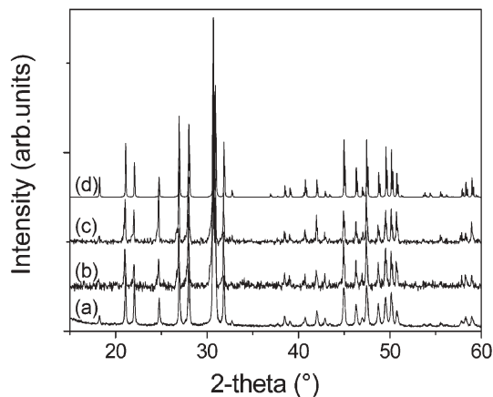
Fig. 2 X-Ray diffraction patterns of \text{La}_{9.33}\text{Si}_6\text{O}_{26} . (a) Nanopowder calcined at 1000 °C/4 h; (b) sample sintered by SPS at 1200 °C/3 min; (c) sample sintered by SPS at 1500 °C/18 min; and (d) theoretical diagram as calculated from ref. 11.
